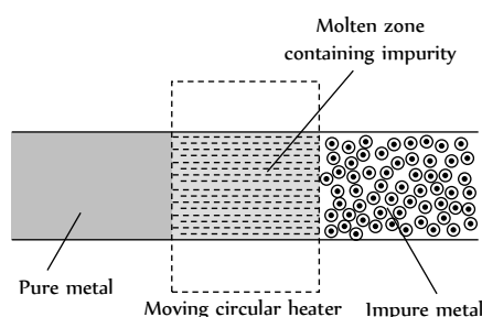
Fig. 16.4. Zone refining of metals
