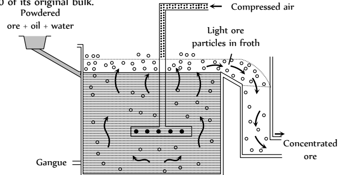
Fig. 16.2. Froth floatation process
