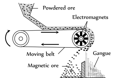
Fig. 16.3 Electromagnetic separation
